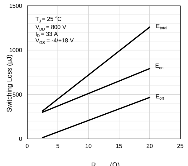
Figure 23: Clamped Inductive Switching Energy vs. R_G(ext)
