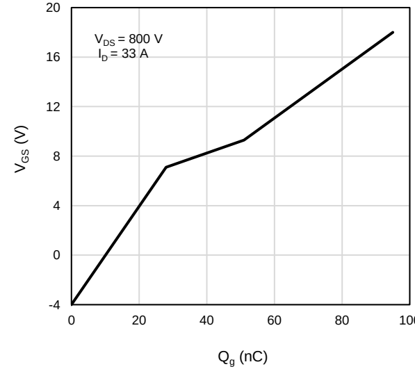
Figure 12: Gate-Charge Characteristics
