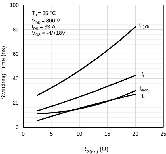
Figure 26: Switching Times vs. R_{G(EXT)}
