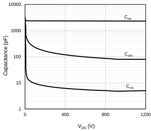
Figure 18: Capacitance Characteristics (0 - 1200 V)
