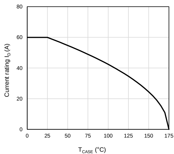
Figure 19: Current De-rating
